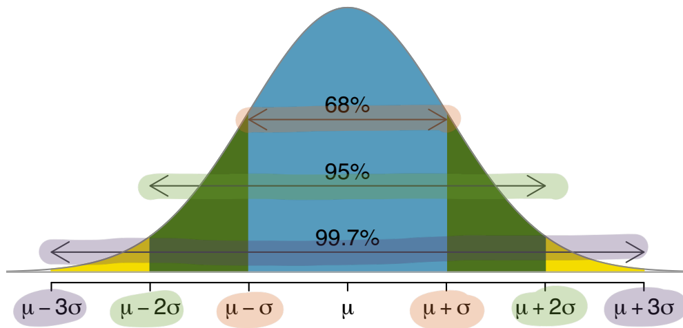
FIGURE 3. Empirical Rule (a.k.a. the 68-95-99.7 rule)
