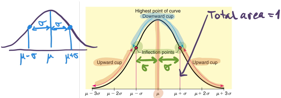
FIGURE 1. Normal (Gaussian) distribution
